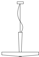
S3 - S33 Ceiling Rose Ø 120 mm Cable 3555 mm Diffuser Ø 680 mm H 445 mm
