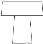
SMALL T1 H 240 mm Diffuser Ø 240 mm Base Ø 112 mm
