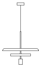
S70 Ceiling Rose Ø 120 mm Cable 3000 mm Diffuser Ø 600 mm H 540 mm
