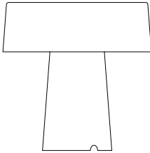
T3 H 480 mm Diffuser Ø 480 mm Base Ø 225 mm
