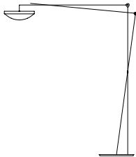
F5 H 2000 mm D 1800 mm Diffuser Ø 400 mm H 120 mm Base Ø 470 mm
