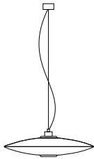
S3 Ceiling Rose Ø 80 mm Cable 2000 mm Diffuser Ø 630 mm
