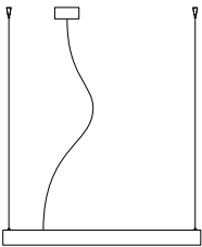
S3 Ceiling Rose Ø 80 mm Cable 2000 mm Diffuser Ø 960 mm H 65 mm
