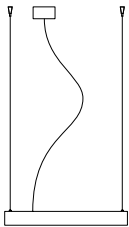
S1 Ceiling Rose Ø 80 mm Cable 2000 mm Diffuser Ø 660 mm H 65 mm
