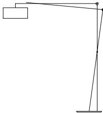
F50 H 2000 mm D 1800 mm Diffuser Ø 420 mm H 180 mm Base Ø 470 mm
