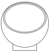
F5 Diffuser Ø 450 mm D 300 mm Base Ø 200 mm H 60 mm
