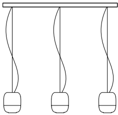
S1 3B Ceiling Rose 40x40x1200 mm Cable 2000 mm Diffuser Ø 180 mm H 210 mm
