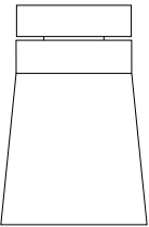
C3 H 215 mm Ceiling Rose Ø 120 mm Diffuser Ø 150 mm
