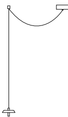
S1L Ceiling Rose Ø 120 mm H 40 mm Lateral Ceiling Attachment Ø 15 mm H 25 mm Cable 3000 mm Diffuser Ø 120 mm H 76 mm
